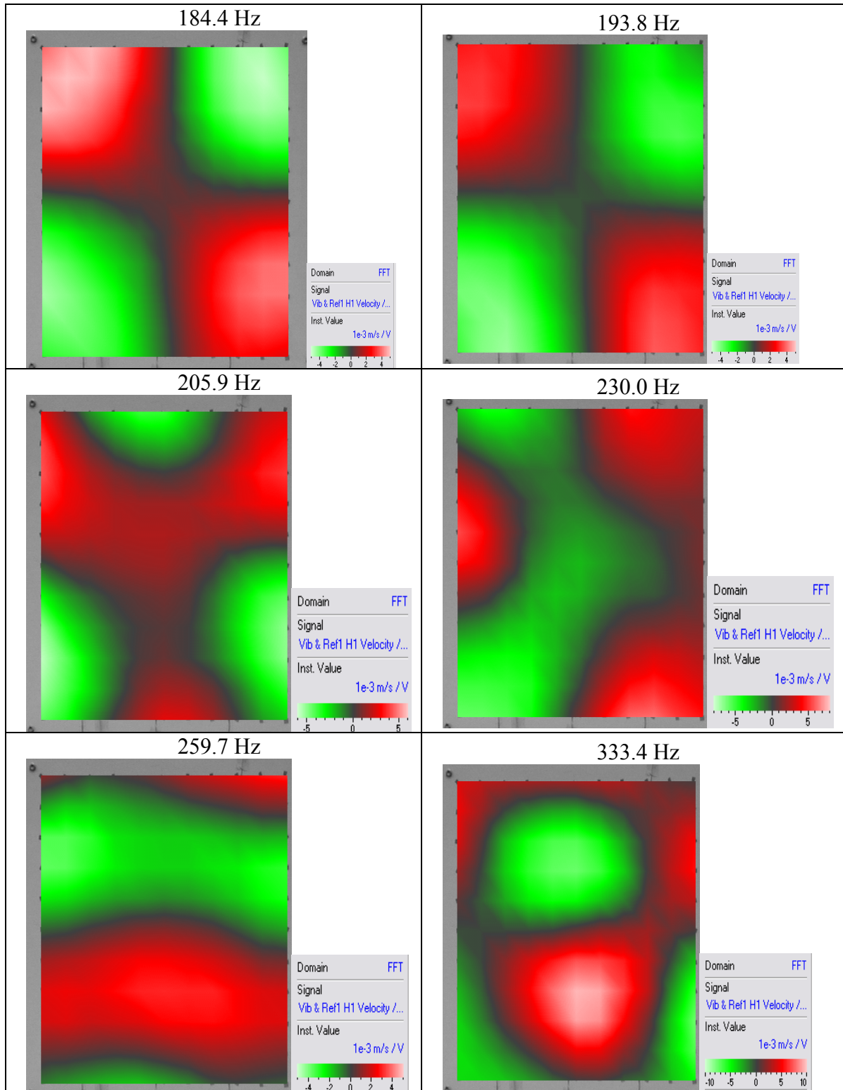
Fig. 18: Responses of the trim panel with open loop control units at resonance frequencies.
