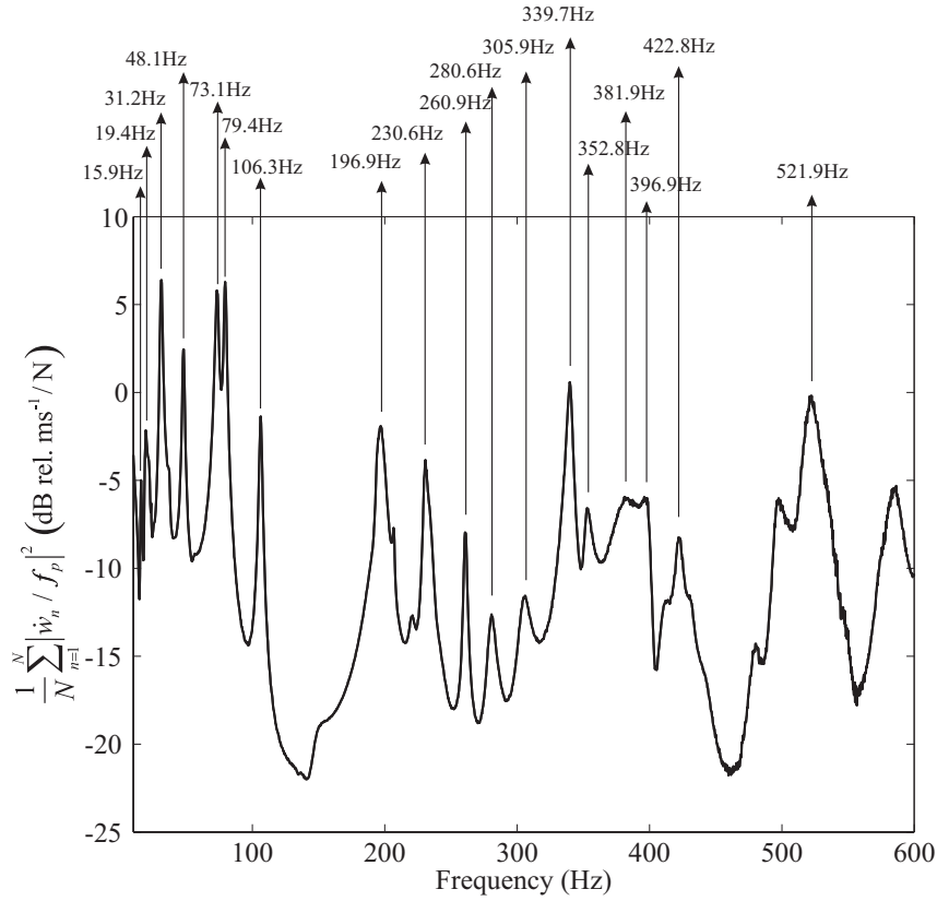
Fig. 13: Spatially averaged FRF of the trim panel without control units per unit force excitation.
