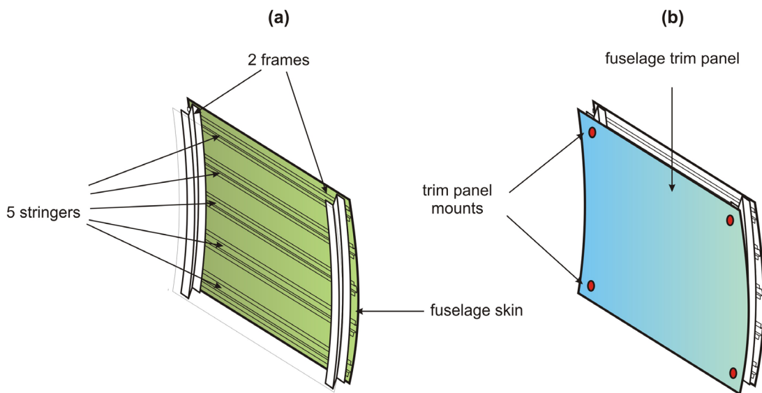
Fig. 1: Sketch of the fuselage section. (a) Green fuselage section composed of two frames and five stringers. (b) Trim panel fixed on four mounts.
