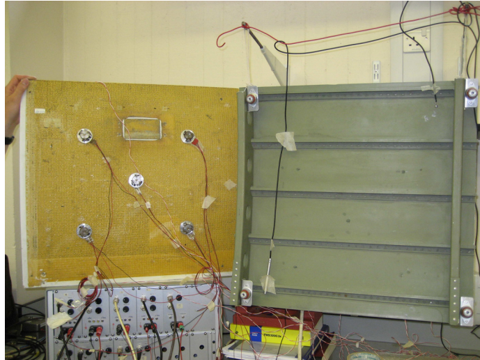
Fig. 6: Front view of the fuselage section and trim panel with five control actuators bonded on the interior side.
