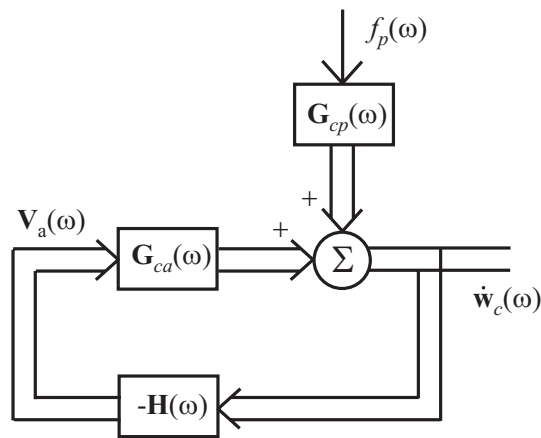
Fig. 10: Block diagram of the multichannel feedback control system implemented on the trim panel
