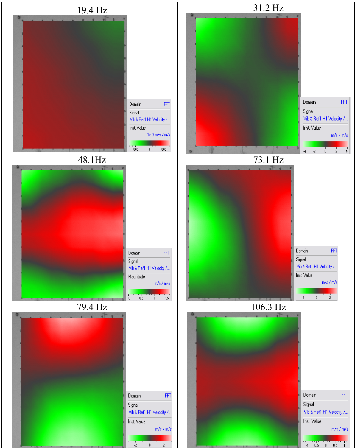
Fig. 14: Responses of the trim panel without control units at resonance frequencies.
