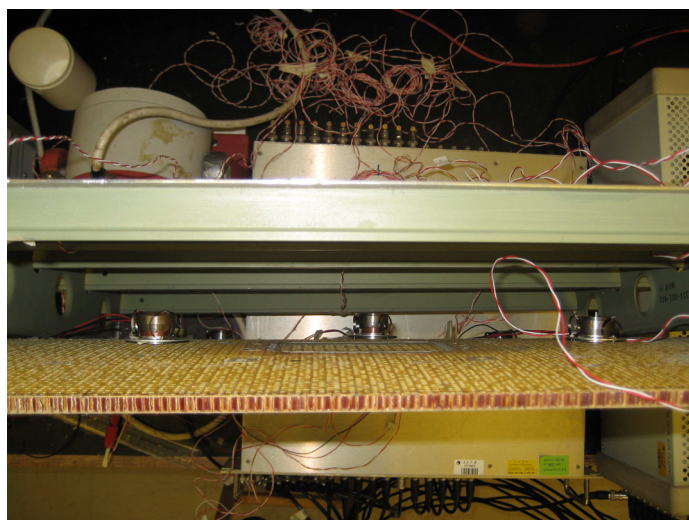
Fig. 8: Top view of the fuselage section and trim panel with five actuators bonded on the interior side.
