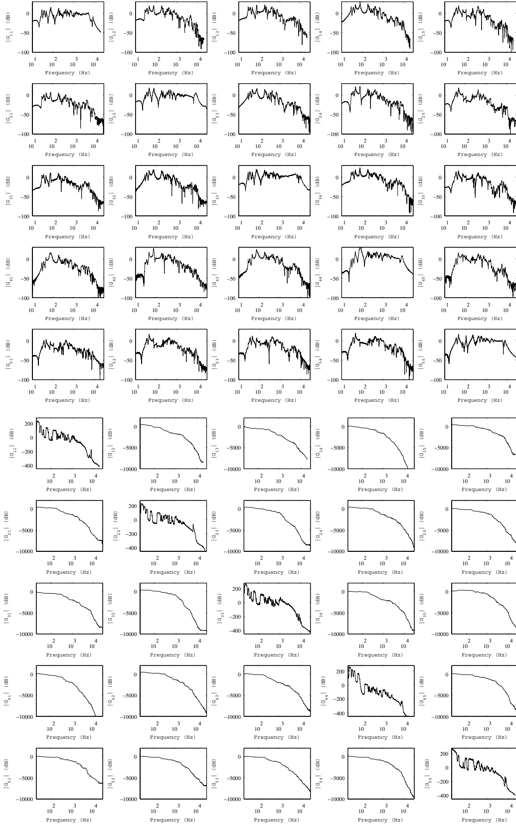
Fig. 11: Amplitude and phase of the measured FRFs between the five error sensors and five inputs to the controllers driving the actuators.
