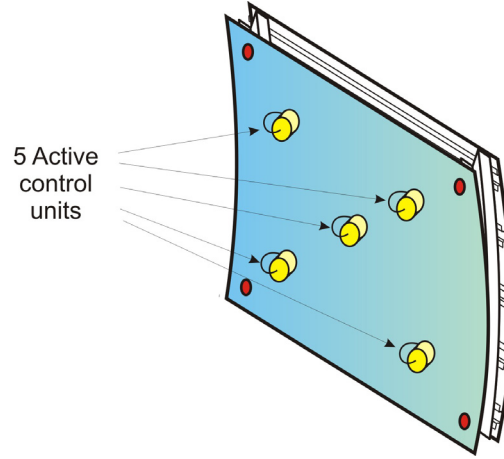
Fig. 5: Fuselage section with the five control units.
