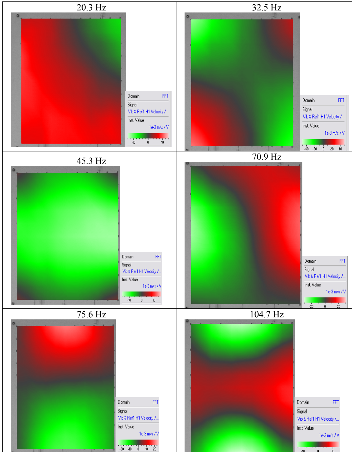
Fig. 17: Responses of the trim panel with open loop control units at resonance frequencies.
