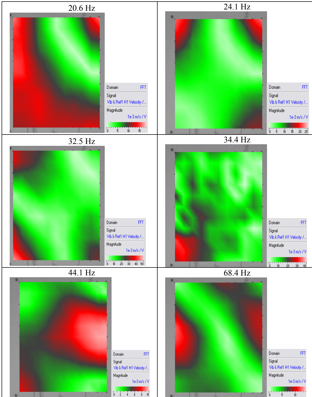
Fig. 20: Responses of the trim panel with closed loop control units at resonance frequencies.
