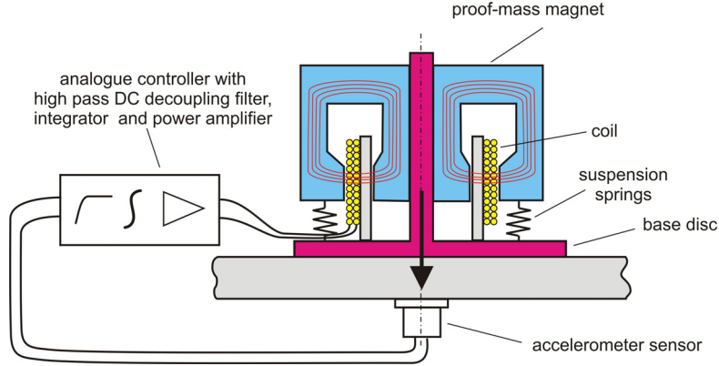
Fig. 3 Sketch of the active damping control unit composed of a proof mass electromagnetic actuator, an accelerometer sensor and an analogue controller.
