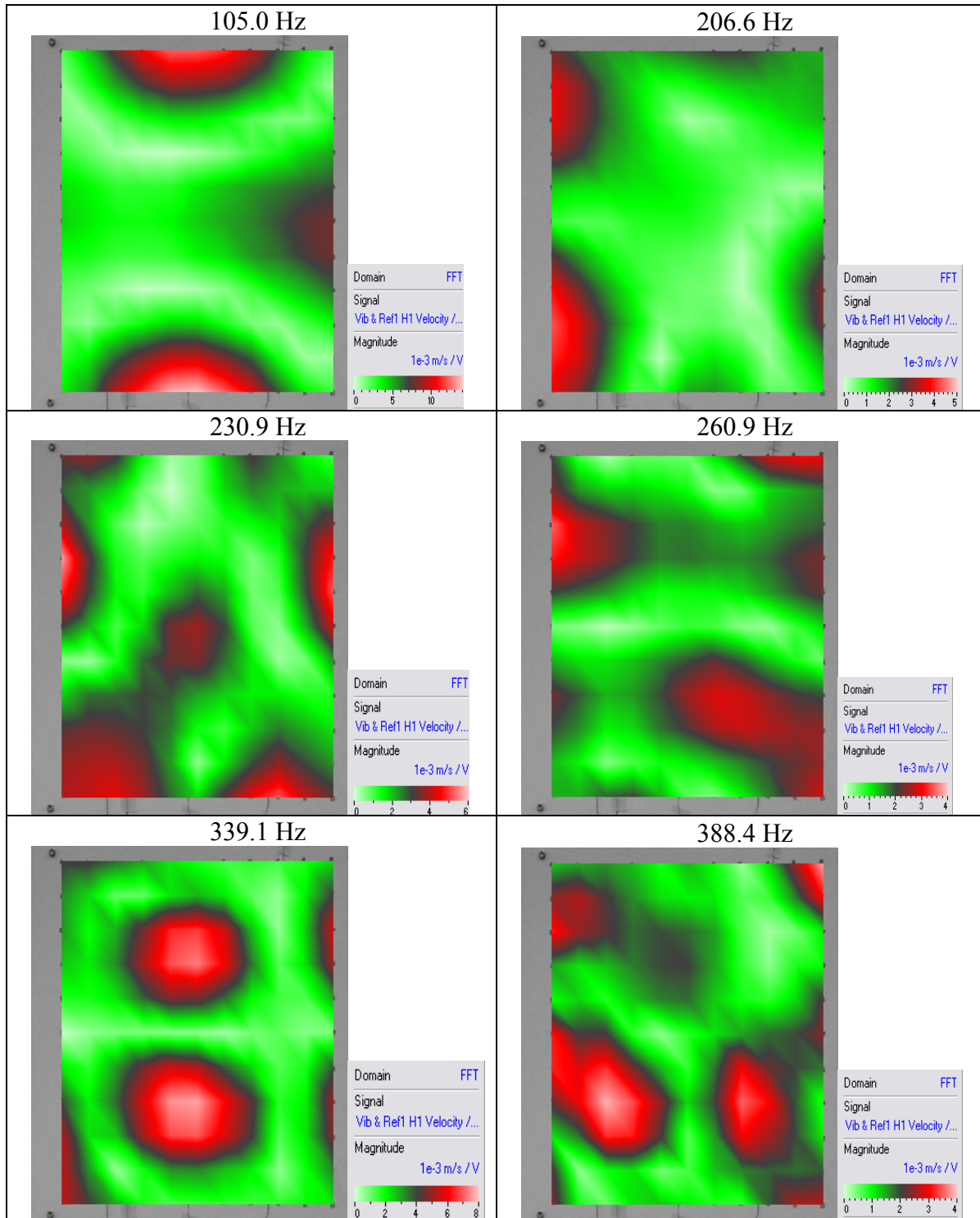
Fig. 21: Responses of the trim panel with closed loop control units at resonance frequencies.
