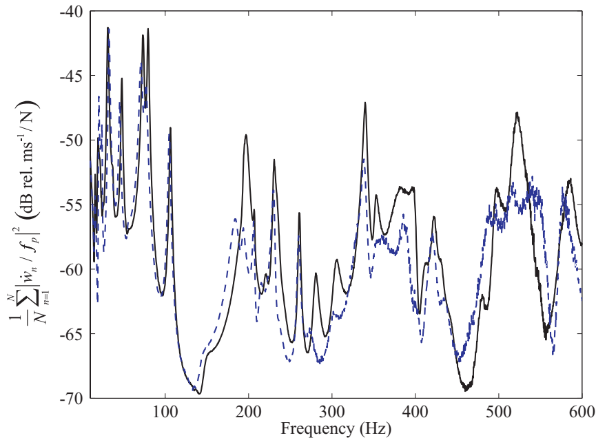
Fig. 16: Spatially averaged response of the trim panel per unit force excitation. Solid-black line without control units, dashed-blue line with open loop control units.
