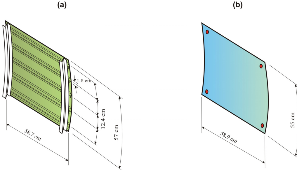
Fig. 2: Principal dimensions of the fuselage double wall.
