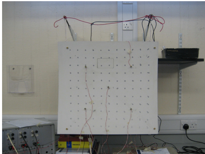
Fig. 7: Front view of the fuselage section and trim panel with five accelerometers bonded in correspondence to the centre of the actuators footprints.
