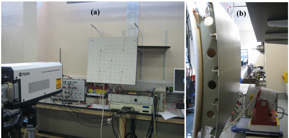
Fig. 9: Measurement setup with laser vibrometer and shaker primary actuator. (a) Front view, (b) lateral view.
