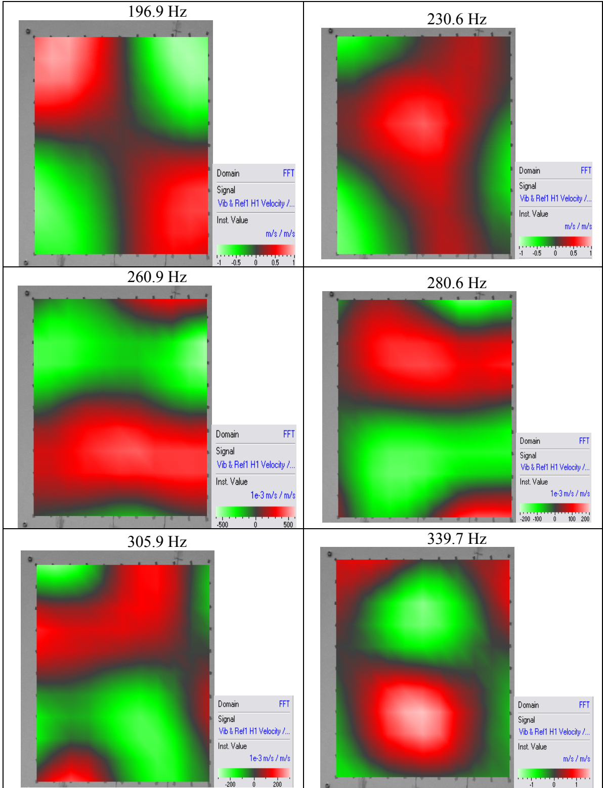
Fig. 15: Responses of the trim panel without control units at resonance frequencies.
