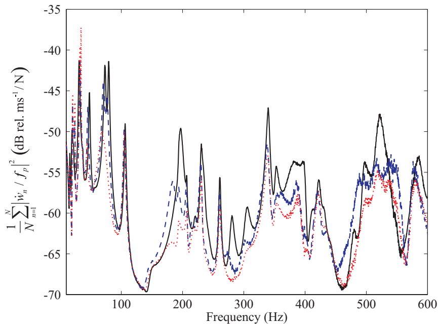
Fig. 19: Spatially averaged response of the trim panel per unit force excitation. Solid-black line without control units, dashed-blue line with open loop control units, dotted-red line with closed loop control units.
