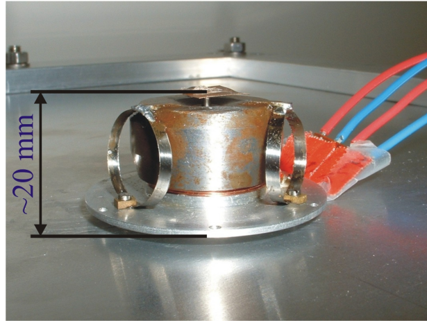
Fig. 4: Photo of the electrodynamic proof mass actuator.
